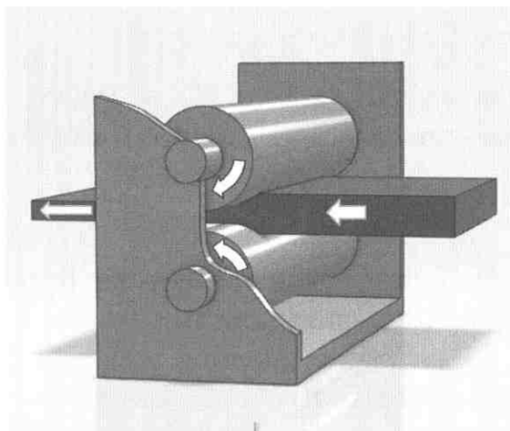
Figure 1- Principe du laminage
